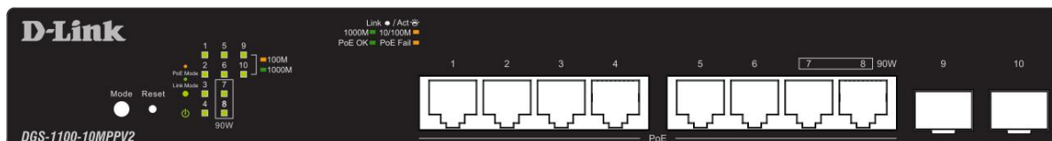
Figure 2-9 – DGS-1100-10MPPV2 Front Panel
